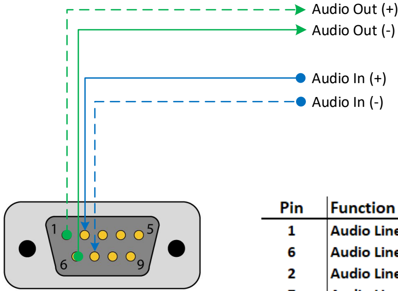
DB-9M Connector
