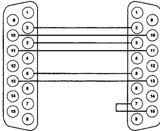
INTERCONNECT CABLE BETWEEN THE AB-100 AND A MATRIX PLUS PORT
