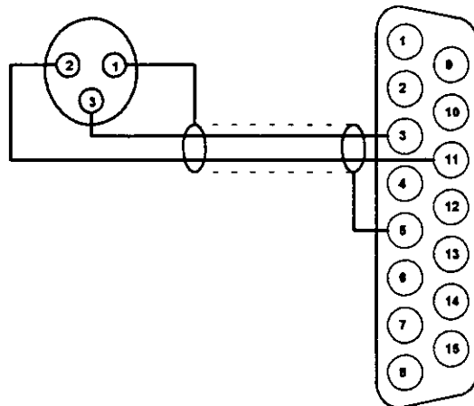
IFB INTERCONNECTCABLE BETWEEN THE AB-100 AND A MATRIX PLUS PORT
