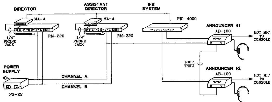
AB-100 Connected To A Clear-Com Party-line System
