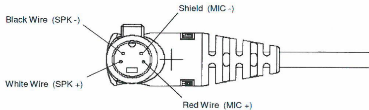
Adapter Mini-DIN Cable 115G363
